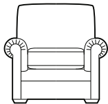
CHAIR H94cm W94cm D95cm SH51cm SW44cm SD56cm AH62cm
